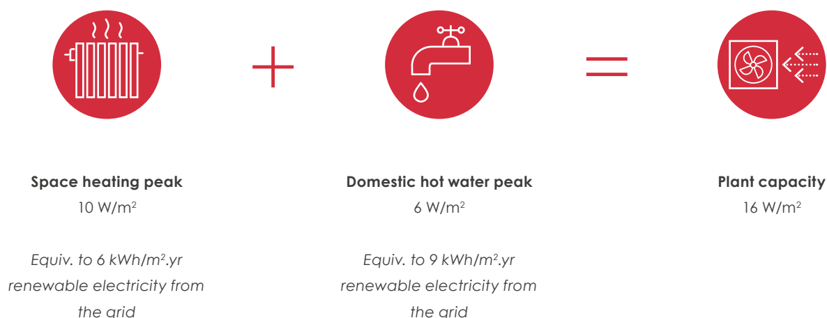
Figure 3.3 - Plant capacity calculation
