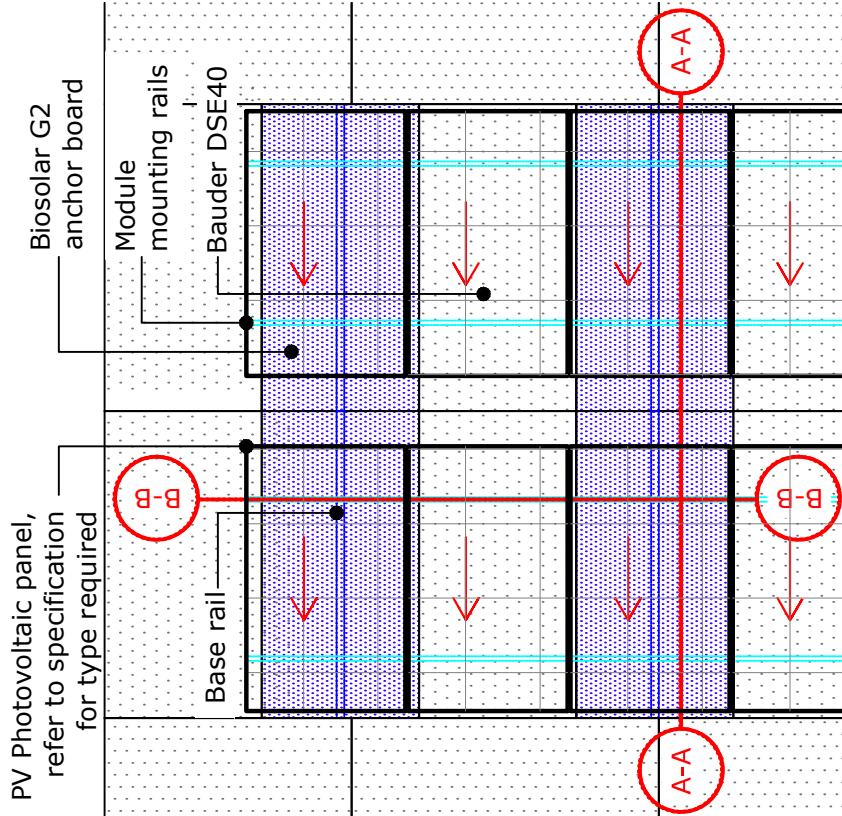
BauderSOLAR G Light Module Section - Top Elevation - Scale 1:50
